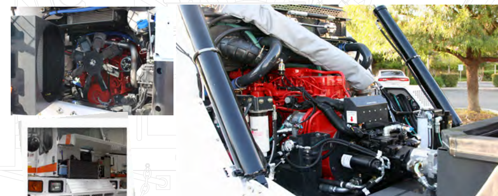
ABOVE The Global M4 features many maintenance-friendly attributes, such as a rear swing-out radiator, easy access front mounted AC condenser, brake and windshield washer fluid reservoirs, and cab fresh air filter.
